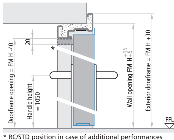
Doors without lower threshold - Vertical cross section
